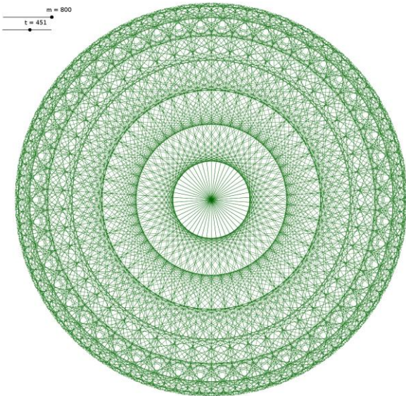
m = 800 ; t = 451
