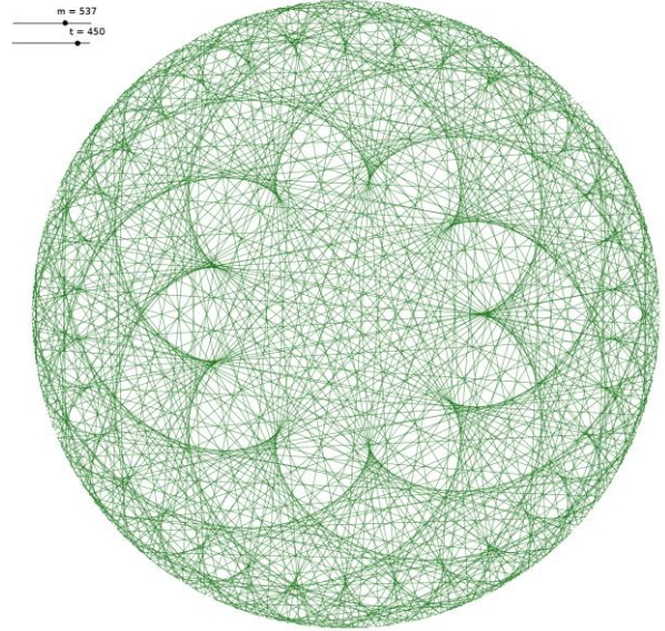
m = 537 ; t = 450
