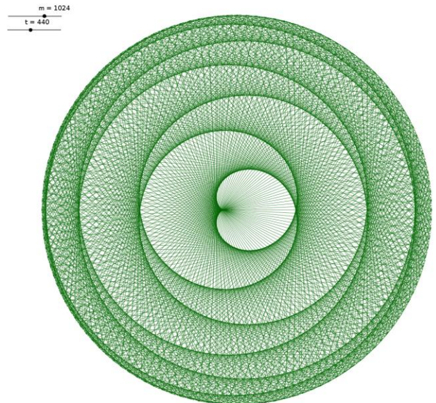
m = 1024 ; t = 440
